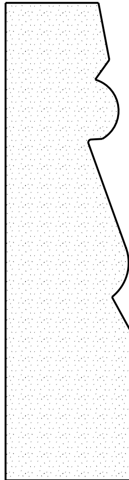
F-1095 1 5/16" X 5"
