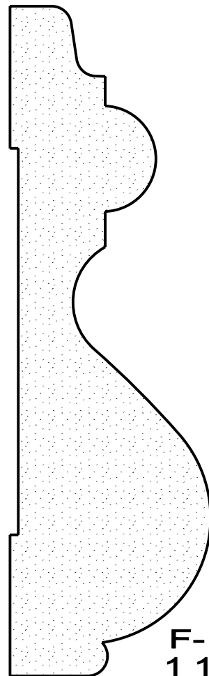
F-1089 1 11/16" X 3 1/8"
